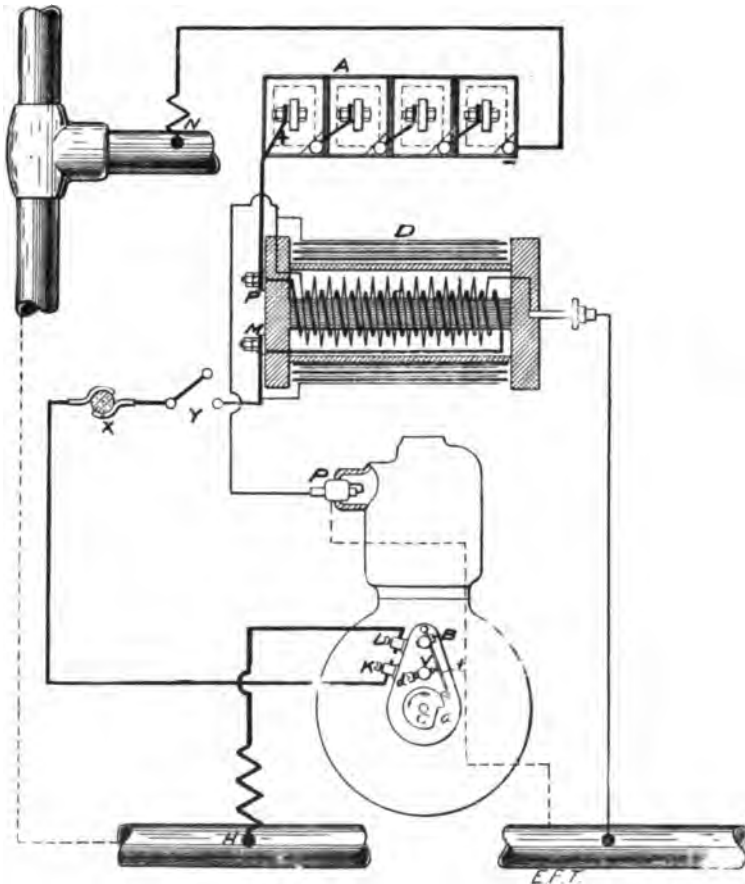
FIG. 332.—Diagram of the De Dion Jump-Spark Ignition Circuit. A is a battery of four cells, one pole of which is connected, as shown, to the tubular frame of the carriage at the point, N, the circuit being thus completed through the steel frame work to binding post, L, on the circuit breaker: thus, the circuit is made by the contact of the trembler, T, with the point of the screw, D, on the post, V, through binding post, K to M, thus through the primary winding of the induction coil and to the opposite pole of the battery. The secondary circuit joined to one pole of the condenser, D, is connected to one end of the sparking plug, P, the other, being grounded to the frame, completes the circuit by the metallic contacts with the body of the motor, as indicated by the dotted line.
